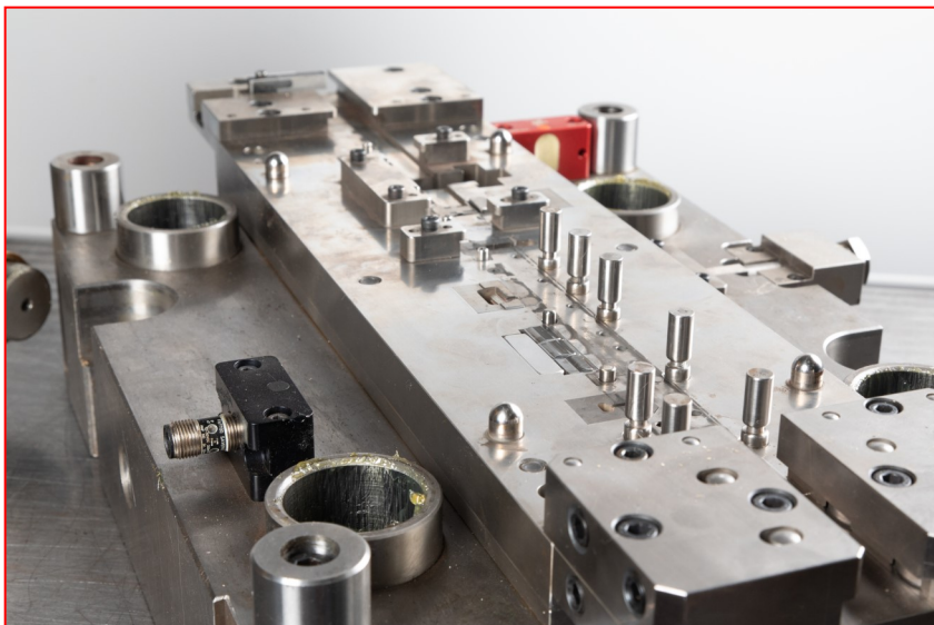
▶ Progressive tool
