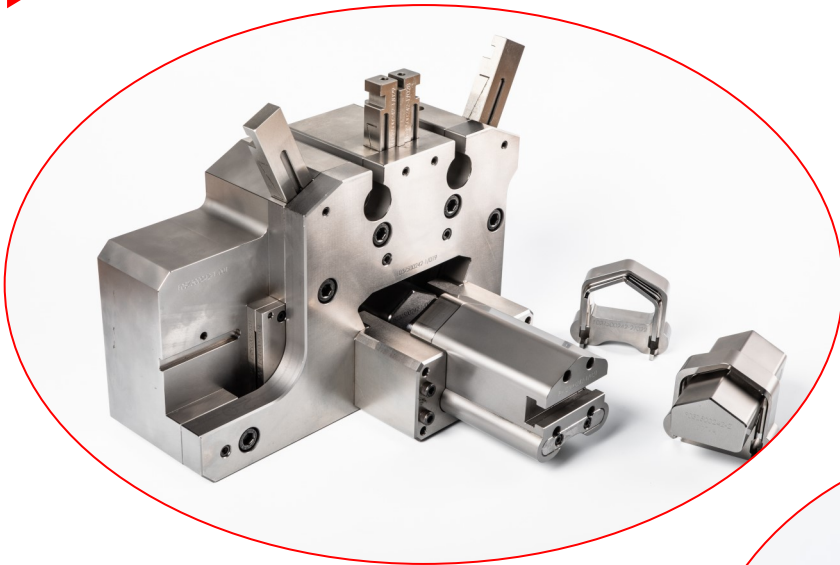
▶ Multi-slide tool
