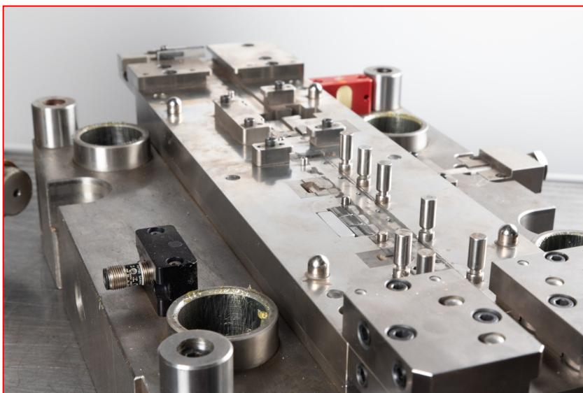
▶ Outil progressif
