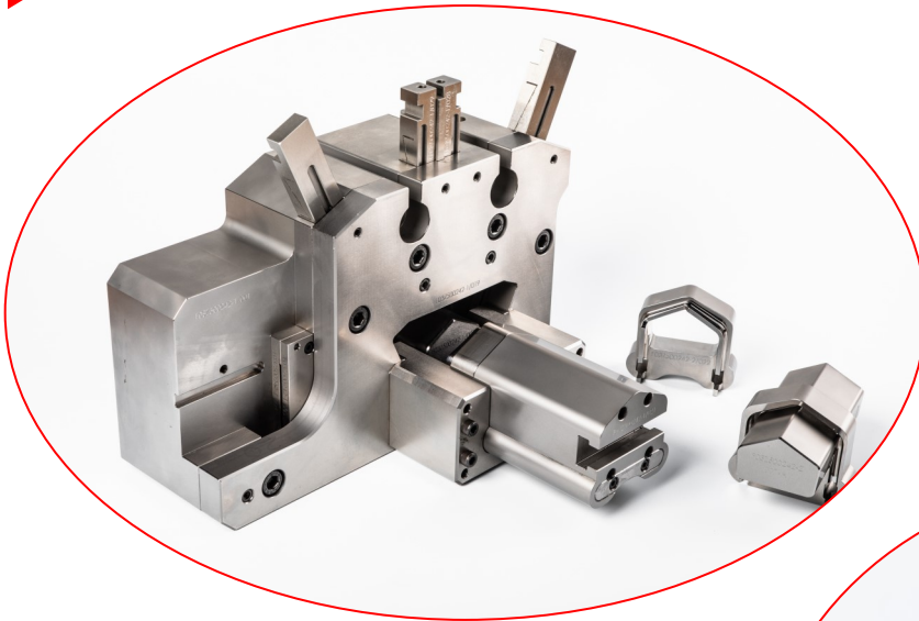
▶ Outil coulisseau
